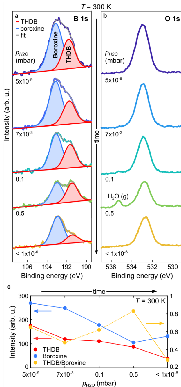
Fig. 3. In-situ NAP-XPS characterization of mixed boroxine and THDB monolayer upon water vapor exposure. (a,b) B 1s and O 1s spectra acquired at T = 300 K upon sequential increase of p_{\text{H}_2\text{O}} and after cell evacuation. Photon energy = 650 eV. (a) Individual components obtained by fitting procedure are superimposed as solid peaks. (c) Absolute intensities of the two B 1s components of panel (a) and their intensity ratio are plotted versus p_{\text{H}_2\text{O}} .
