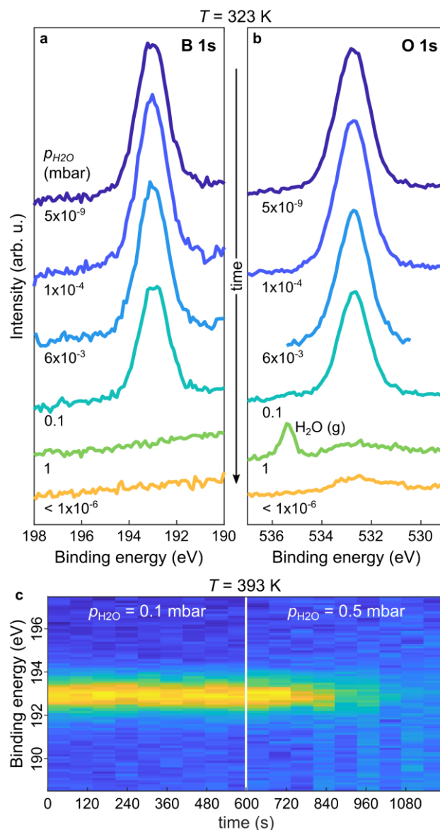
Fig. 2. In-situ NAP-XPS characterization of hydrolysis in the boroxine framework upon water vapor exposure. (a,b) B 1s and O 1s spectra of boroxine framework on Au(111) upon sequential exposure to increasing p_{\text{H}_2\text{O}} (shown in shades of blue and yellow) and after cell evacuation (indicated in orange) at T = 323 \text{ K} . The water gas-phase peak, \text{H}_2\text{O}(\text{g}) , is indicated. (c) Contour plot of B 1s spectra acquired during exposure of the boroxine framework to water vapor pressures at T = 393 \text{ K} , with p_{\text{H}_2\text{O}} increased from 0.1 to 0.5 mbar after 600 s. Photon energy = 650 \text{ eV} .
