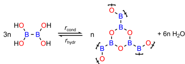
Scheme 1. Reversible condensation reaction of tetrahydroxydiboron (THDB) leading to a 2-dimensional boroxine ( B_3O_3 ) framework. The rates for condensation ( r_{\text{cond}} ) and hydrolysis ( r_{\text{hydr}} ) are indicated.
