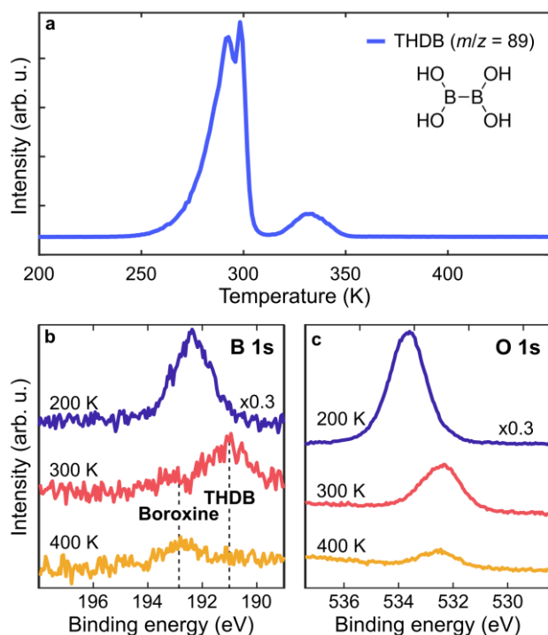
Fig. 1. On-surface formation of the boroxine framework in UHV. (a) TPD measurement for the intact THDB molecule ( m/z = 89 amu, linear heating rate of 1 \text{ K s}^{-1} ). (b,c) B 1s and O 1s spectra of THDB/Au(111) after initial multilayer deposition at 200 K (blue), and after annealing to 300 K (red) and 400 K (orange), respectively. Photon energy = 1253.6 \text{ eV} .
