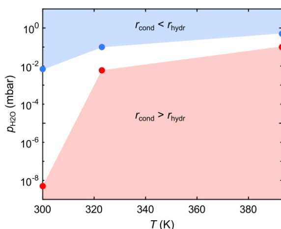
Fig. 4. Pressure-temperature diagram of the reversible condensation reaction of tetrahydroxydiboron (THDB) leading to a 2D boroxine framework. The regions where the rates of the condensation ( r_{\text{cond}} ) and hydrolysis ( r_{\text{hydr}} ) reactions become dominant are indicated in red and blue, respectively.
